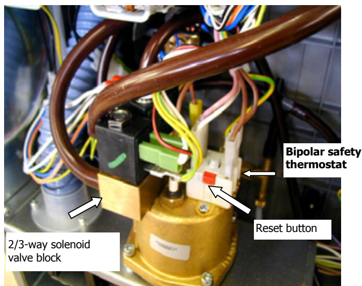
Back view of boiler detail
