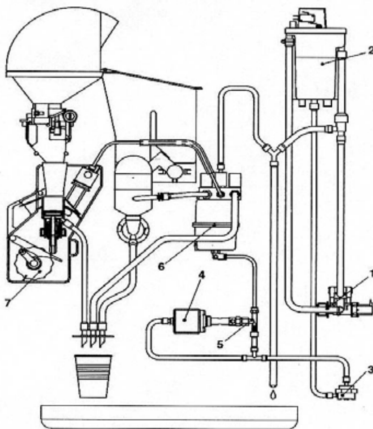
HYDRAULIC LAYOUT - "ESPRESSO" VERSION
