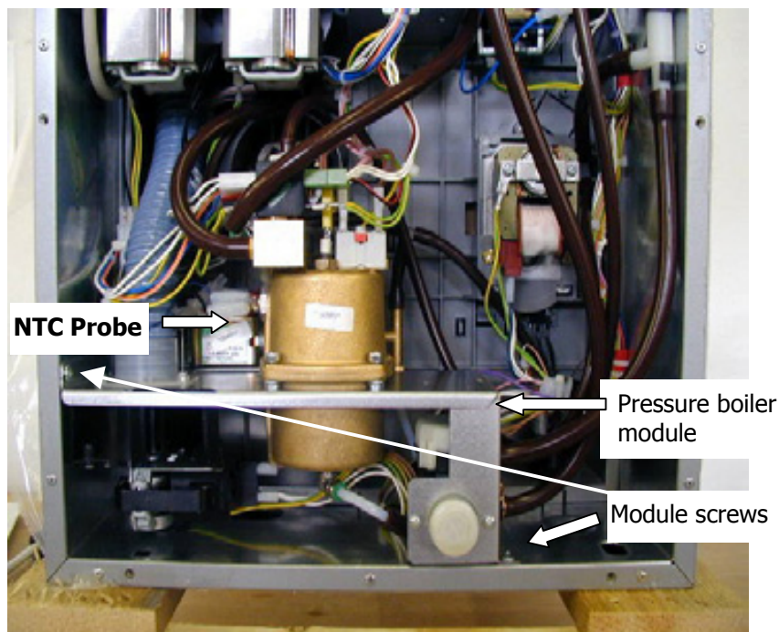
Back view of boiler detail
